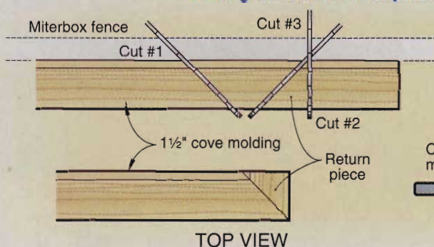
DRAWING 1 Cutting the cove return piece
